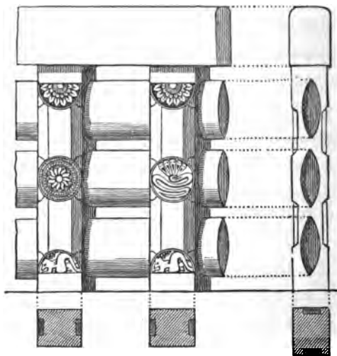
RAIL AT SANCHI.
